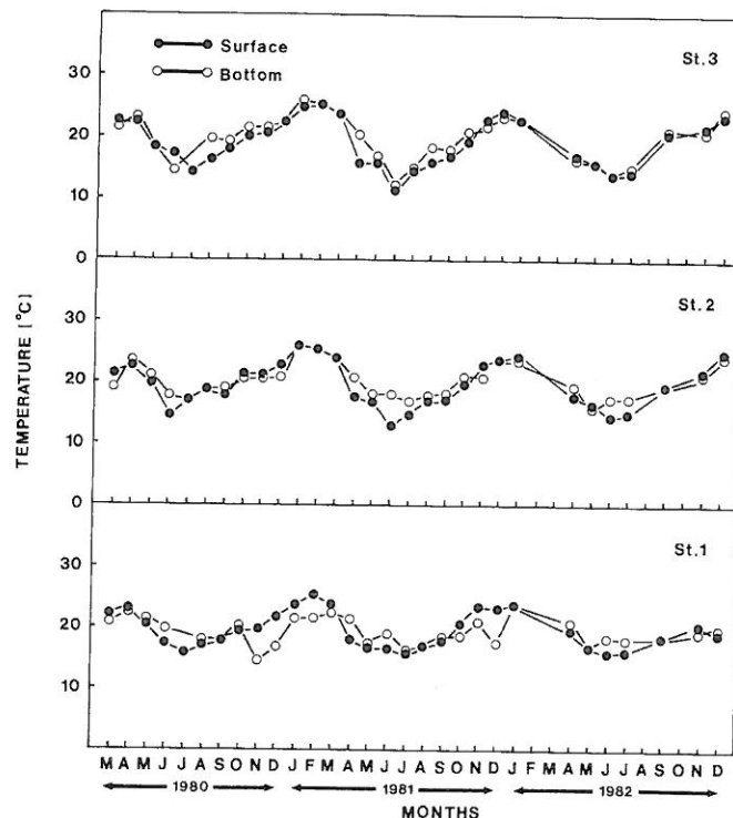
Figure 3 Monthly temperatures ( ^{\circ}\text{C} ) recorded at three Stations in the Mbashe estuary.
