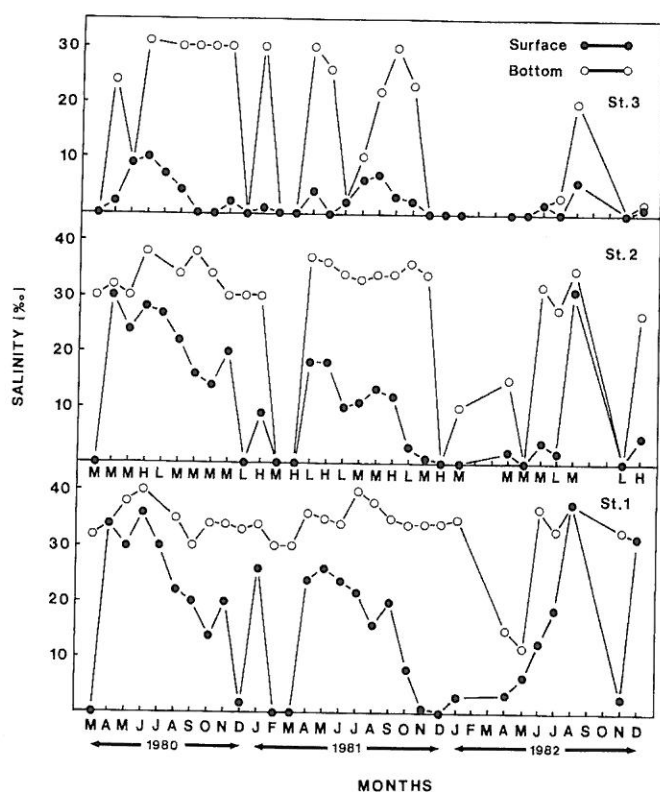
Figure 4 Monthly salinities (‰) recorded at three Stations in the Mbashe estuary (H – high tide, M – mid-tide, L – low tide).
