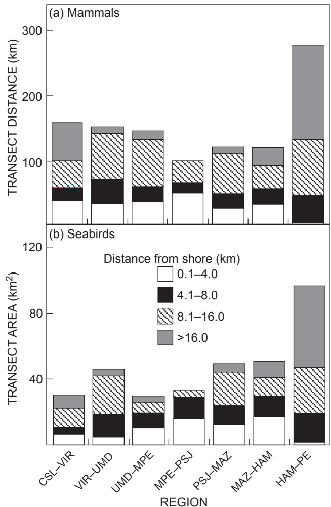
Figure 2: (a) Total mammal survey transect distance and (b) seabird survey transect area covered during the survey per block and distance from shore class. The locations follow the regional divisions shown in Figure 1
